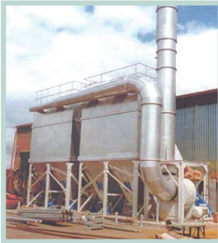
Fume extraction from hot-dip galvanizing process
