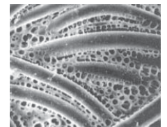
Ravlex PTFE surface
