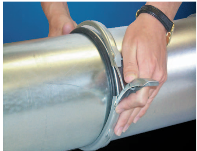
Snap QF clamp over O-ring and one end of slip duct.
