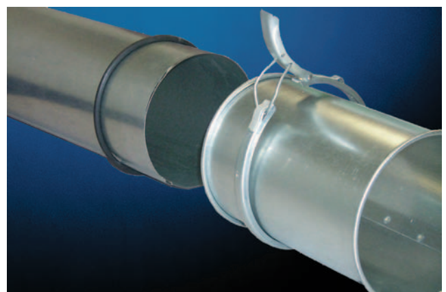
Snap QF clamp over O-ring and one end of slip duct.
